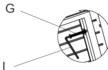
DETAIL 2-2
